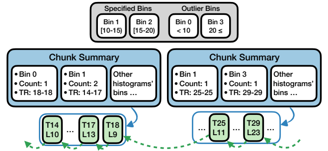
Figure 8: A detailed view of the chunk summaries in Figure 7. Summaries contain statistics for records in a chunk that fall in an index-specific histogram bin. Loom constructs a summary for the active chunk, but the summary is not accessible to queries. When the active chunk fills up, Loom writes the summary to the chunk index and makes it available for queries.
